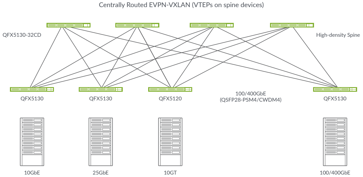
Figure 2: QFX5130-32CD as a 100GbE/400GbE ToR in a typical cloud data center
