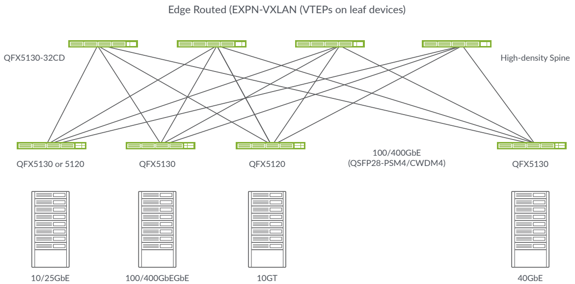
Figure 3: Private cloud data center with the QFX5130-32CD as high-density spine
